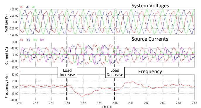
Fig. 4 – Voltage, current and frequency response for the system without Shunt Power Compensator.
