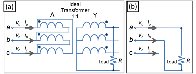
Fig. 2 - Example of an unbalanced resistive circuit: (a) Circuit like presented in [16]; (b) Equivalent circuit.
