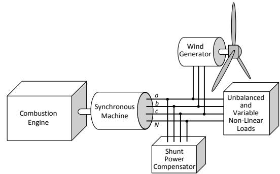
Fig. 3 – Simulated micro-grid with a combustion engine / generator, wind generator, unbalanced nonlinear loads and a Shunt Power Compensator.
