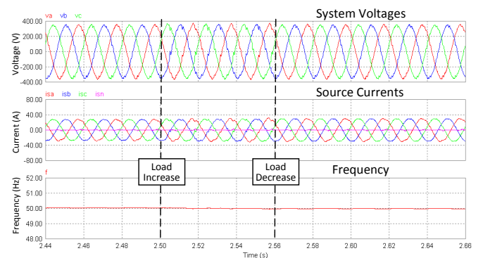
Fig. 5 – Voltage, current and frequency response for the system with Shunt Power Compensator.
