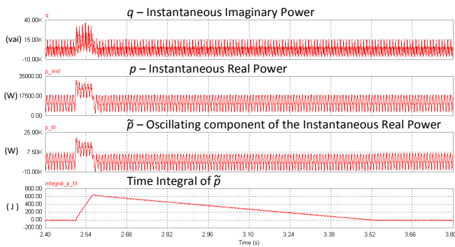
Fig. 6 – q , p , \tilde{p} and time integral of \tilde{p} when load changes (see Fig. 4 and Fig. 5), as calculated by the control system of the Shunt Power Compensator.
