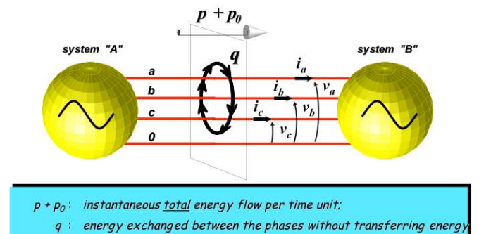
Fig. 1 - Power exchange in a three-phase four-wire system.
