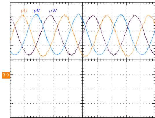
Fig. 16. Output Voltage (100V/div, 5ms)
