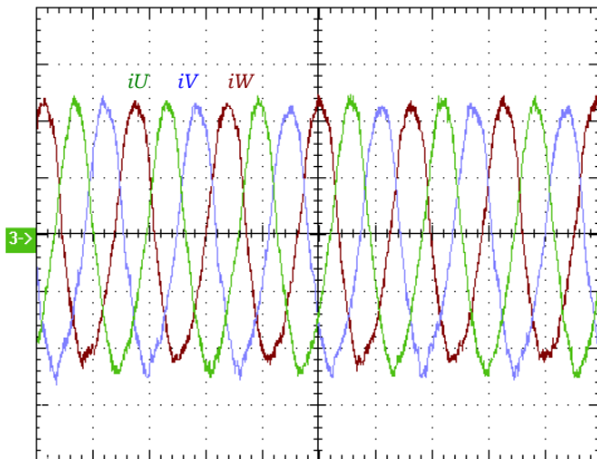
Fig. 18. Motor Current (2A/div, 10ms)
