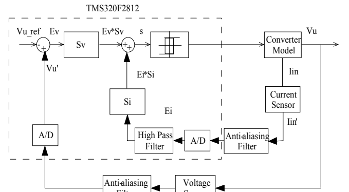
Fig. 5. Control Block Diagram
