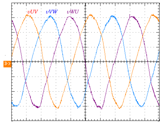
Fig. 20. Line Voltages – 45Hz (100V, 5ms)
