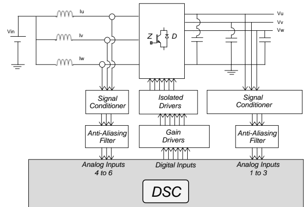
Fig. 15. Converter Block Diagram
