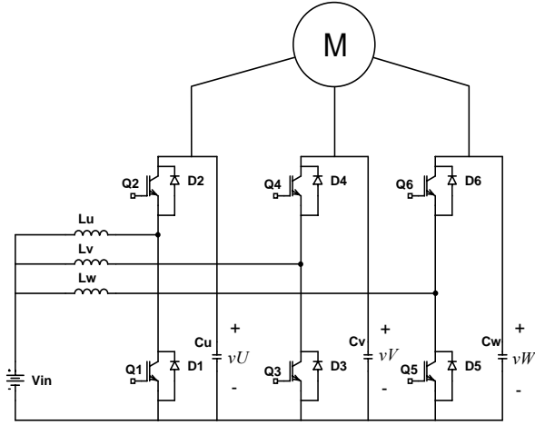
Fig. 3. Three - Phase Boost Inverter
