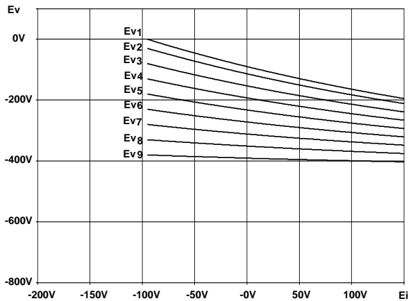
Fig. 6. Structure 1
