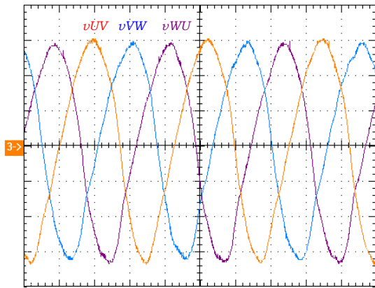
Fig. 17. Line Voltages (100V/div, 5ms)
