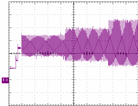
Fig. 22. Soft Start of the Motor (100V/div, 250ms)
