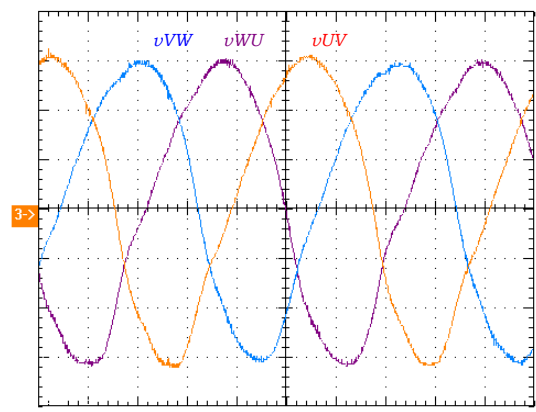
Fig. 21. Line Voltages – 75Hz (100V, 2.5ms)
