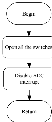
Fig. 11. External Interrupt Flowchart
