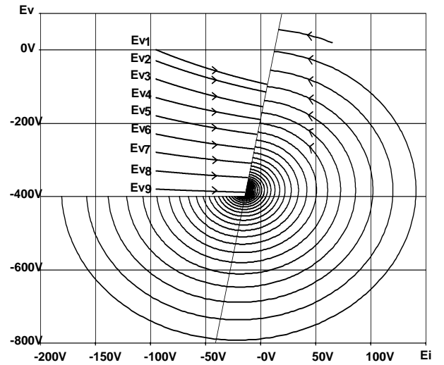
Fig. 8. Combined space-state planes
