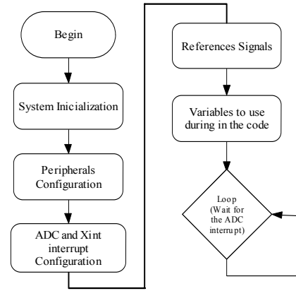
Fig. 10. Main Flowchart
